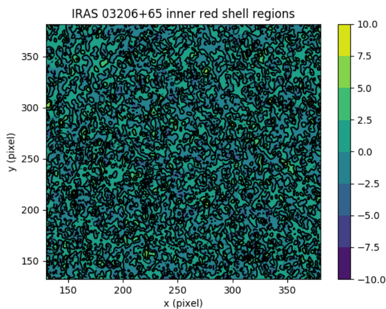
Figure 5.21 Color contour intensity map of IRAS 03206+6521 centered on the IRAS source at 1612MHz of the red inner region. Velocity 8.3 km/s (star's reference frame). Pixel scale: 1 pixel is 1.2 arcsec. Intensities are in millijansky.
