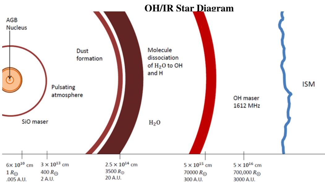
Figure 1.2 Simplified 2-D schematic of different shell layers and their approximate locations surrounding an OH/IR star.
