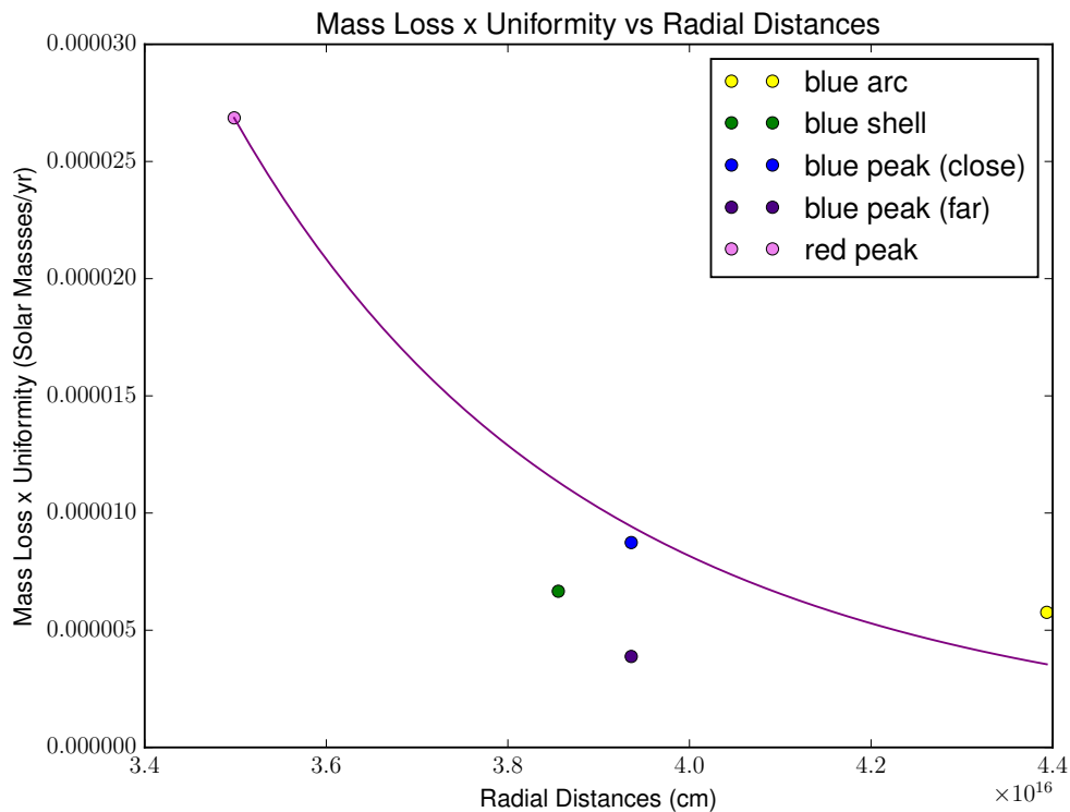
Figure 5.29 Using Netzer's mass loss estimates we weighted them by the uniformity we calculated through different layers in the OH maser shell. The points were weighted according to their detection Gaussian strength above the noise. The regions in the legend are data points from specific regions in the OH maser shell. In the regions where we find the peak of the blue-shifted spectral line we found 2 different maser shells at different radial locations and denote them "close" and "far" with respect to the center of the image.
